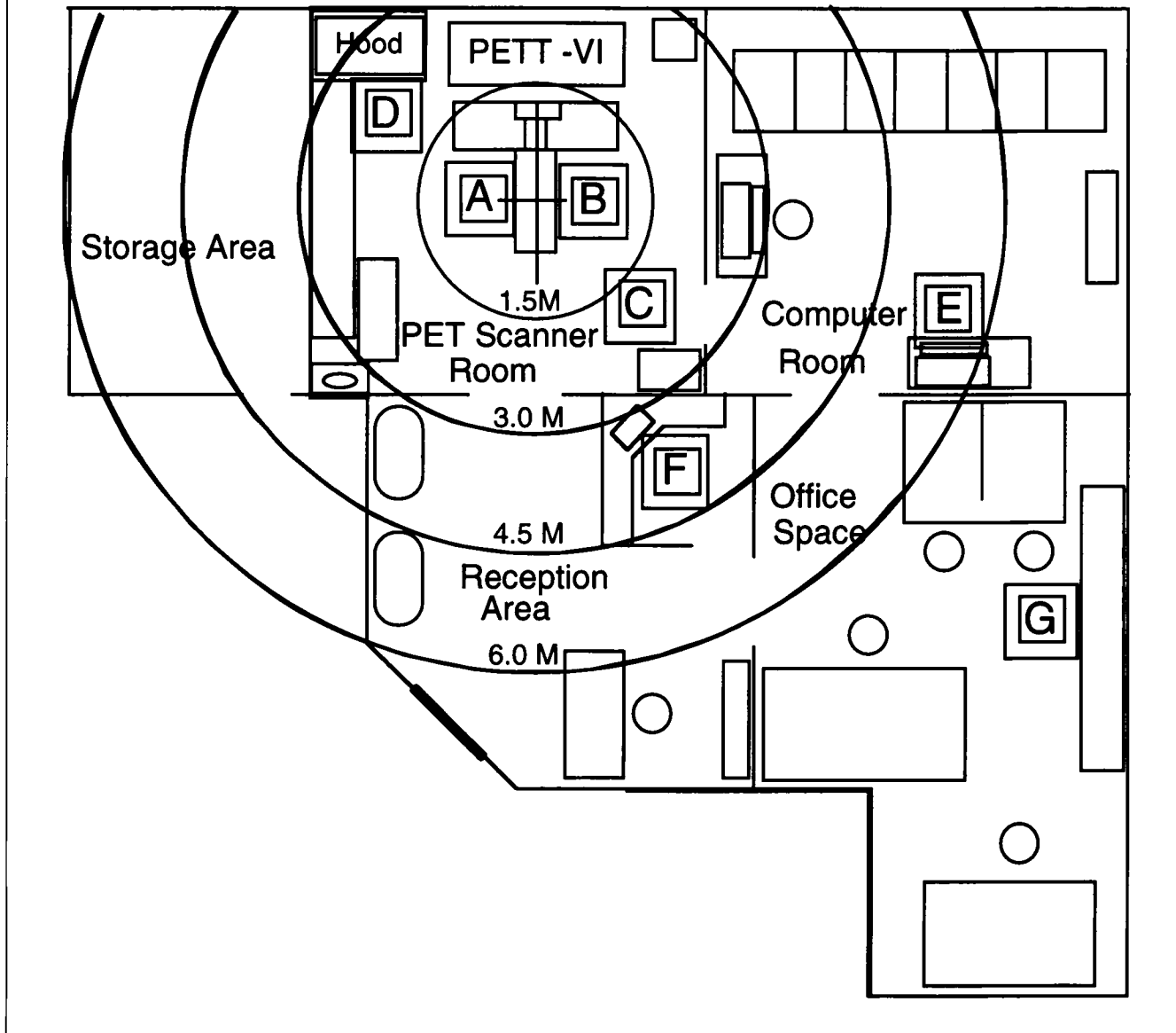
FIGURE 2. A scale drawing of the PET Center at the University of Chicago. The letters indicate the approximate location of the staff involved in a positron tomography study, with the distances from the center of the scanner shown by the circles.
