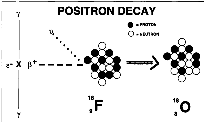
FIGURE 1. Positron decay occurs when an atom has an excess of protons relative to the number of neutrons in its nucleus. A positron is ejected from the nucleus of an atom with an initial energy equal to the difference in nuclear binding energies of these two atoms, less any energy used to eject a second particle from the nucleus which is called a neutrino.
